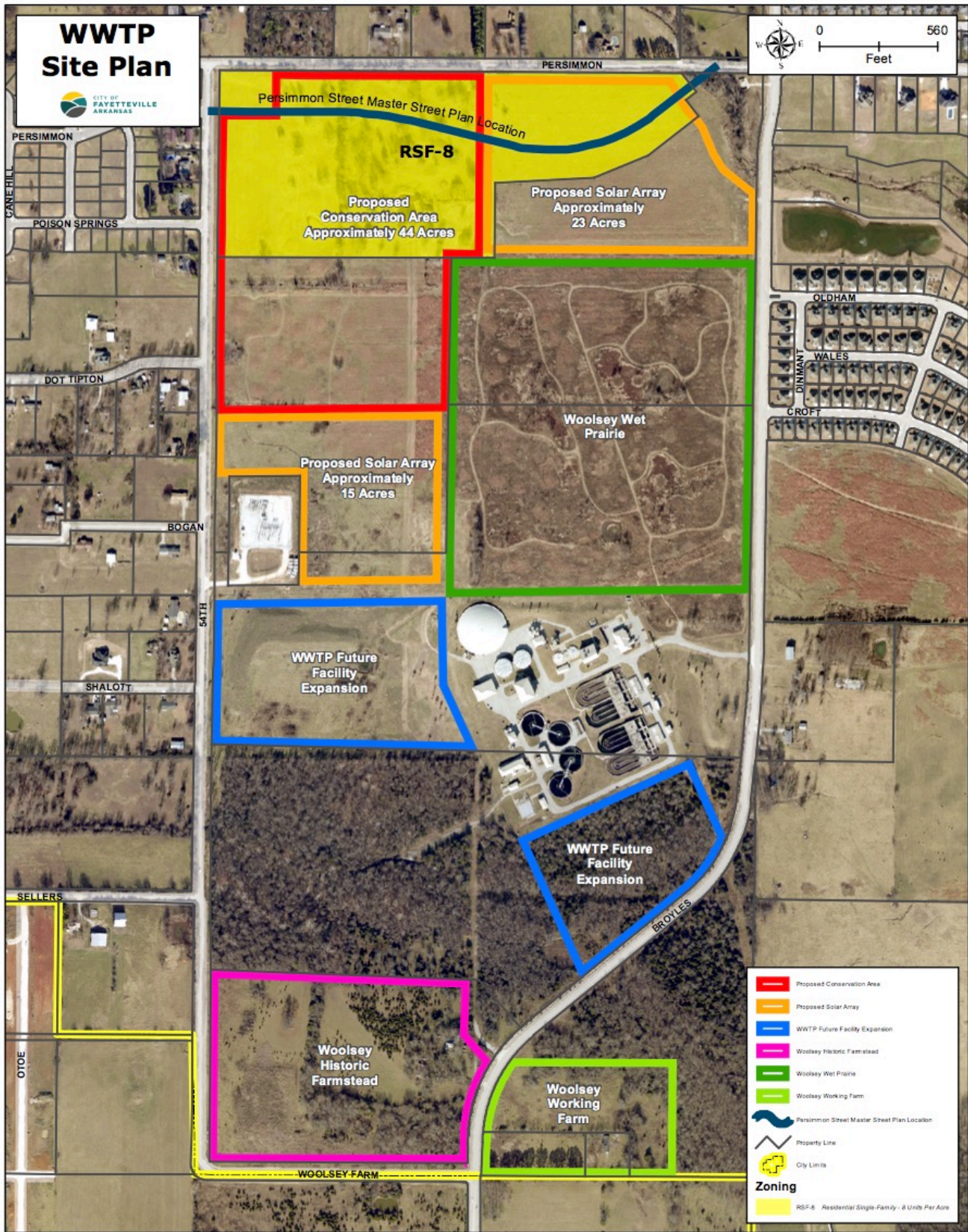
Figure 2 – Conceptual Solar Array Site Plan
